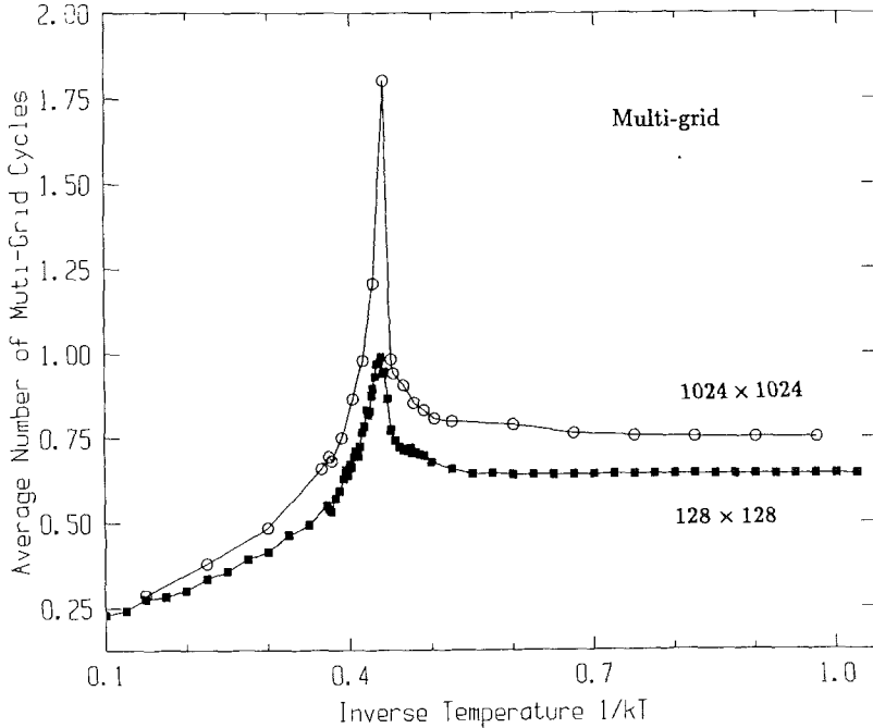
Fig. 5. Average number of relaxation cycles ( D' ) as a function of inverse temperature 1/kT for the multigrid algorithm. Two different lattice sizes are shown: 128 \times 128 and 1024 \times 1024 . The number of cycles is fractional because we test for completion inside the cycle.
