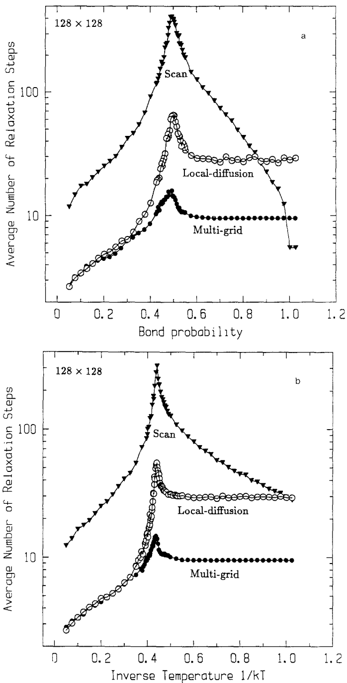
Fig. 3. Average number of relaxation steps for the three algorithms: multigrid, scan, and local diffusion for a 128 \times 128 system. (a) The results for d=2 random bond percolation. (b) The results for the d=2 Swendsen-Wang Ising dynamics. In both cases, at p=0.5 (random percolation) or 1/kT=0.4406868 (Ising), the clusters are fractal and the algorithms exhibit critical slowing down.
